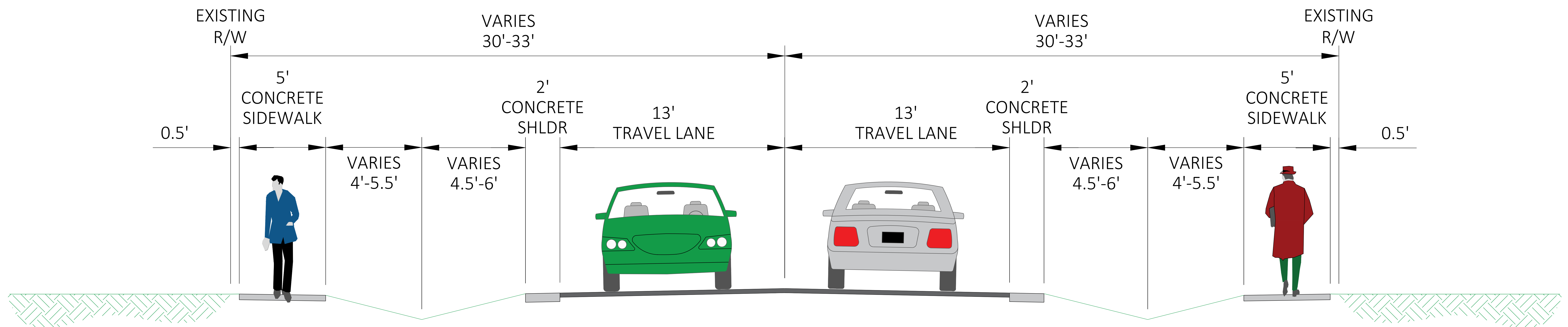
PROPOSED TYPICAL SECTION
