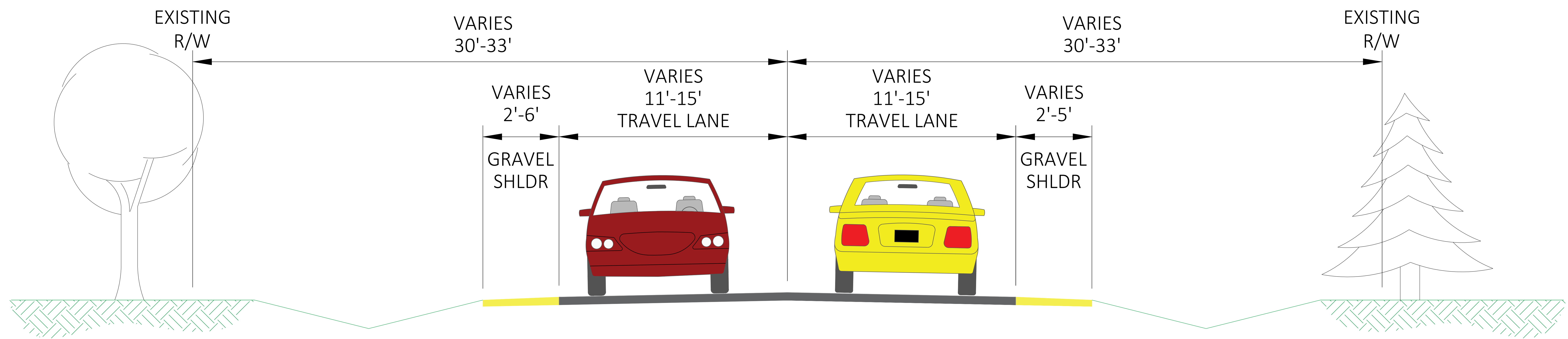
EXISTING TYPICAL SECTION
